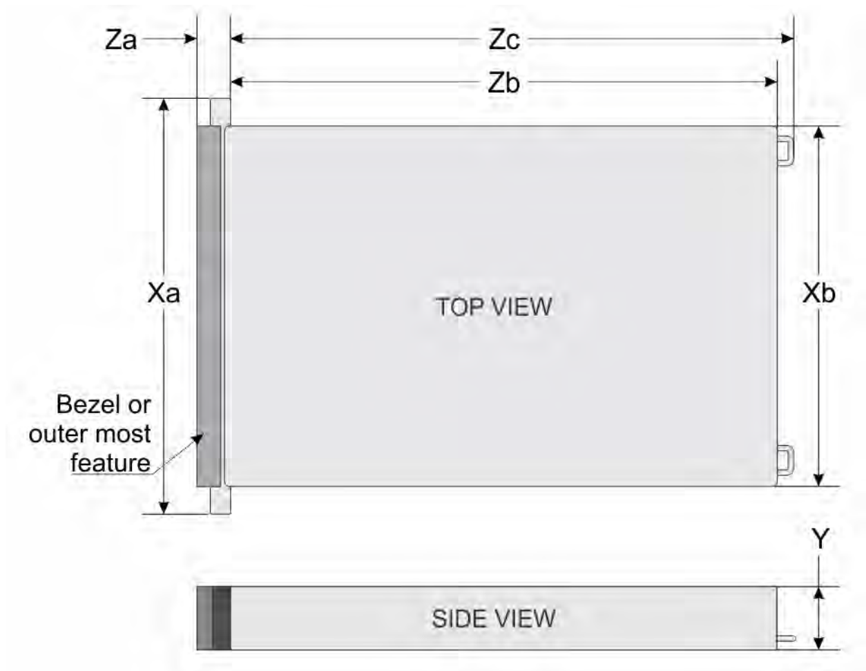
Figure 36. Chassis dimensions
