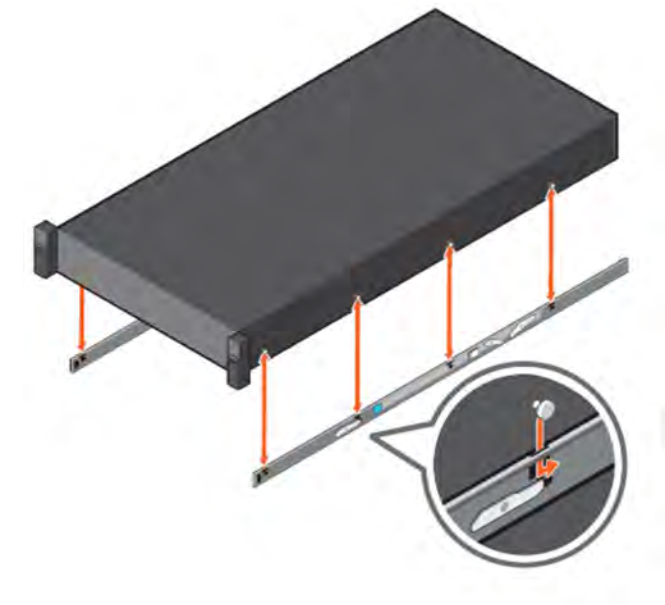
Figure 47. Attach the inner rails to the system
