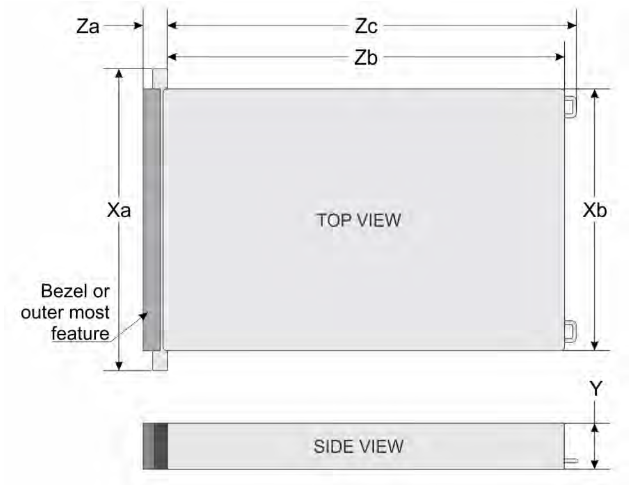
Figure 57. Chassis dimensions
